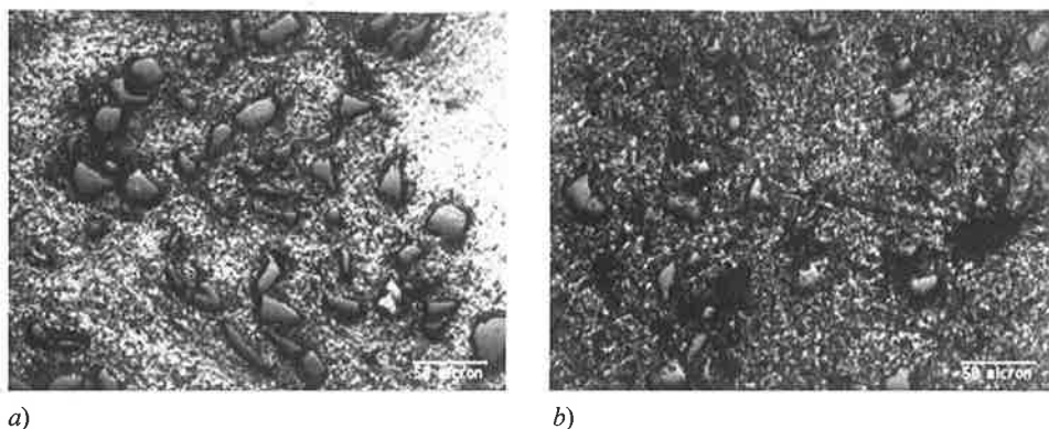
Fig. 2. Metallographic structure of (a) composite material A356/10SiC, (b) A356/10SiC/5Gr hybrid composite
