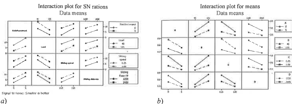
Fig. 4. Interaction factor effect for wear rate of Al composite (a) SN ratio and mean (b)
