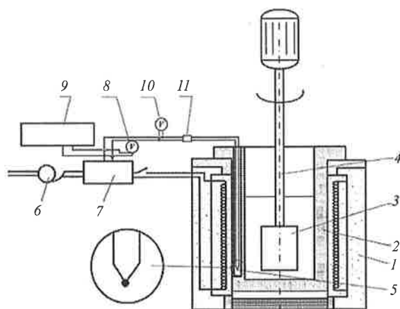
Fig. 1. Schematic drawing of the apparatus for compocasting processing (1 – resistance furnace, 2 – crucible, 3 – mixer, 4 – mixer shaft, 5 – thermocouple and from 6 to 11 – devices and instruments for temperature measurement, control and regulation)
