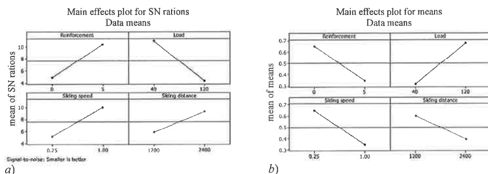
Fig. 3. Main effects plot for wear rate of composites (a) SN ratio and mean (b)
